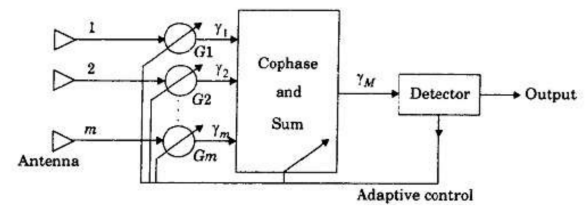
Maximal ratio combiner: weight, co-phase, sum, then detect.
