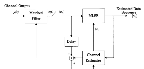
MLSE with an adaptive matched filter and a channel estimator in the loop.
